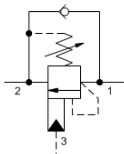
3-Port Non-vented
